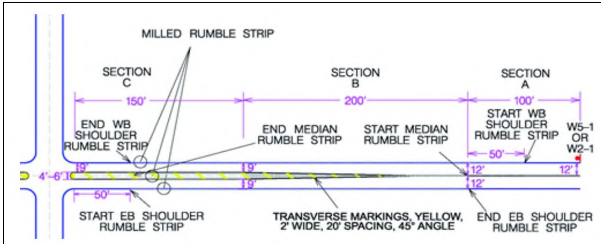
Figure 61. Illustration. Smooth lane narrowing typical design.
